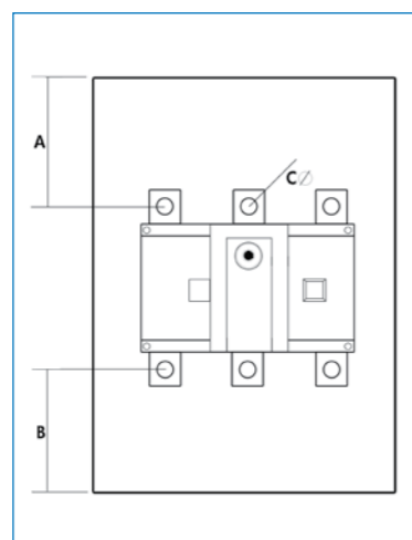
ISOLATOR INTERNAL DIMENSIONS
