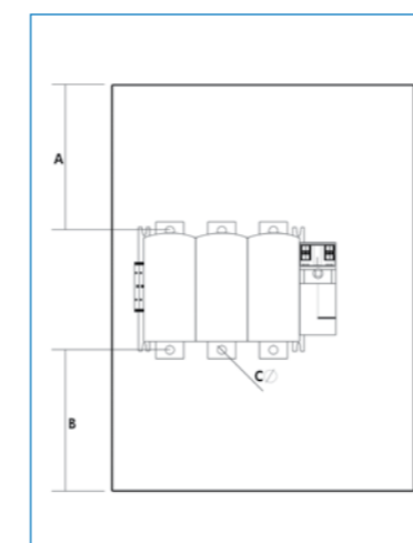
SWITCHFUSE INTERNAL DIMENSIONS
